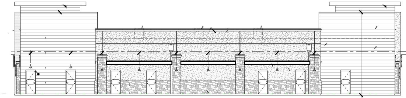
REAR ELEVATION
