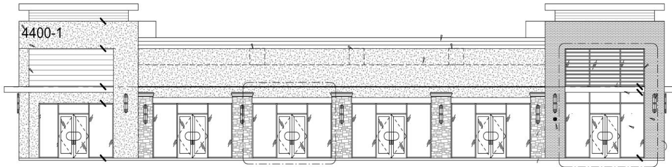
REAR ELEVATION
