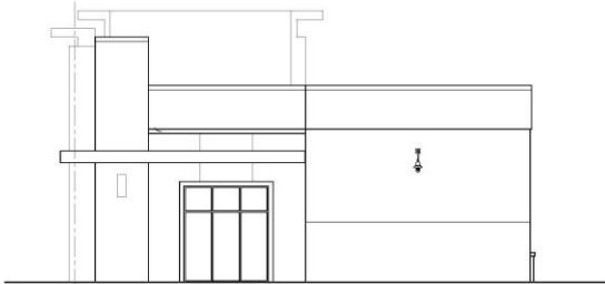
4 RIGHT-SIDE ELEVATION BUILDING 5 SCALE = 1/8"-1'-0"
