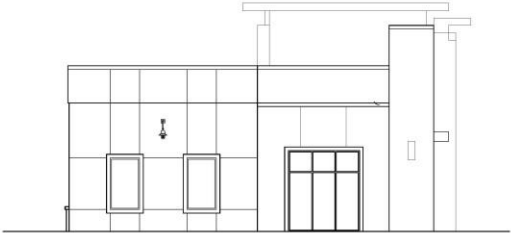
3 LEFT-SIDE ELEVATION BUILDING 9 SCALE = 1/8"-1'-0"
