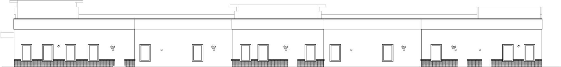
2 REAR ELEVATION BUILDING 9 SCALE = 1/8"-1'-0"
