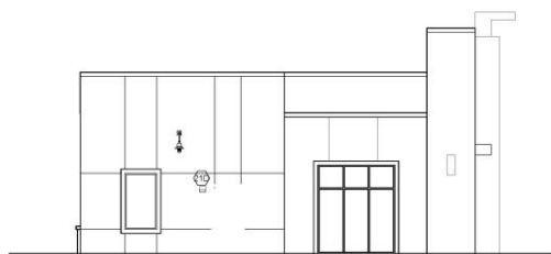
3 LEFT-SIDE ELEVATION BUILDING 10 SCALE = 1/8"-1'-0"
