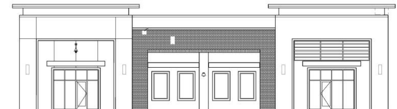
3 LEFT-SIDE ELEVATION BUILDING 8 SCALE = 1/8"-1'-0"
