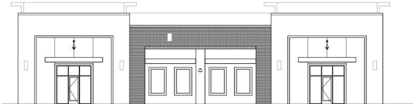
4 RIGHT-SIDE ELEVATION BUILDING 7 SCALE = 1/8"-1'-0"
