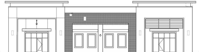
3 LEFT-SIDE ELEVATION BUILDING 6 SCALE = 1/8"-1'-0"
