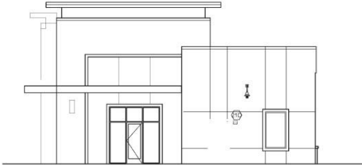
4 RIGHT-SIDE ELEVATION BUILDING 9 SCALE = 1/8"-1'-0"
