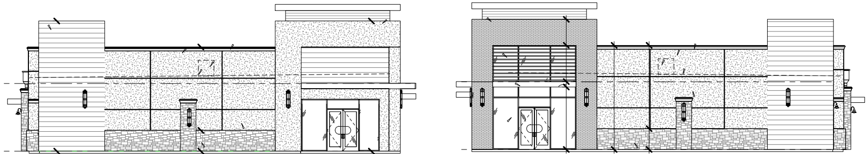
SIDE ELEVATION
